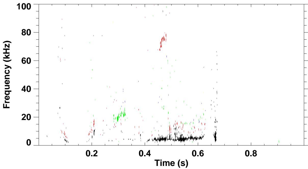
Shot 138496 \omega_B(\omega) spectrum for toroidal mode number: 1 2 3 4 5
