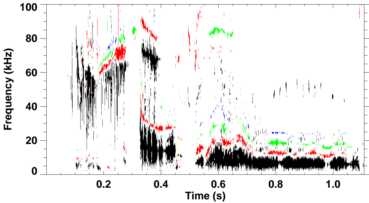
Shot 138640 \omega B(\omega) spectrum for toroidal mode number: 1 2 3 4 5
