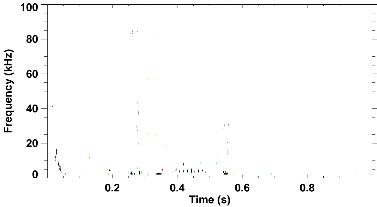
Shot 138682 \omega B(\omega) spectrum for toroidal mode number: 1 2 3 4 5
