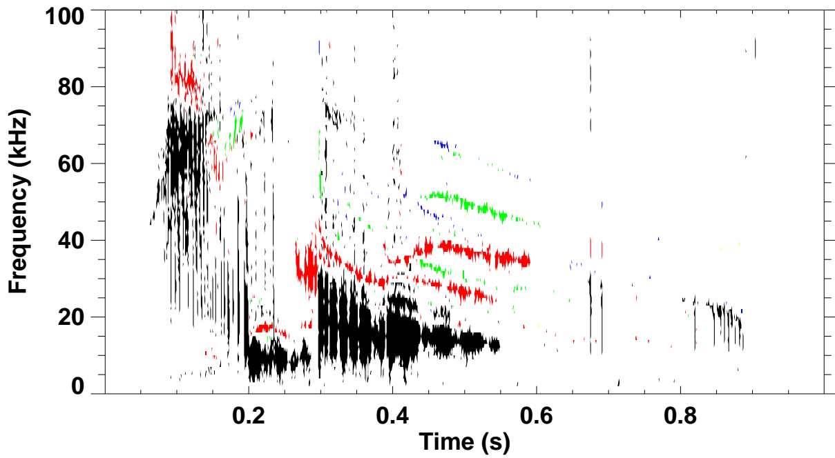
Shot 139046 \omega B(\omega) spectrum for toroidal mode number: 1 2 3 4 5
