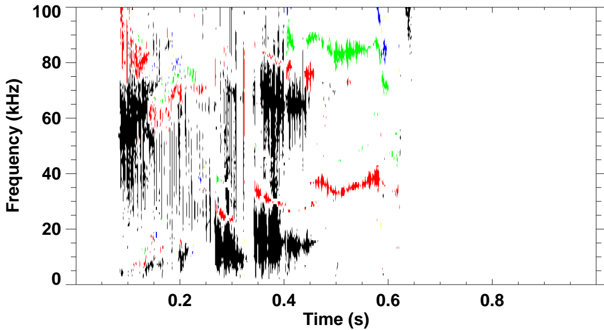
Shot 139376 \omega B(\omega) spectrum for toroidal mode number: 1 2 3 4 5
