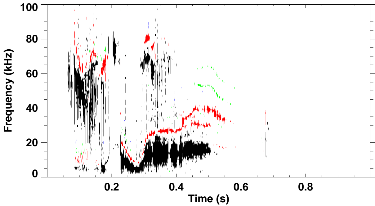
Shot 139455 \omega_B(\omega) spectrum for toroidal mode number: 1 2 3 4 5
