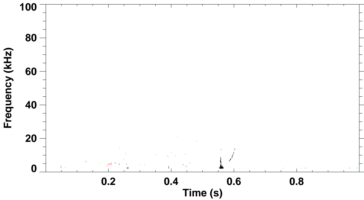
Shot 139529 \omega_B(\omega) spectrum for toroidal mode number: 1 2 3 4 5
