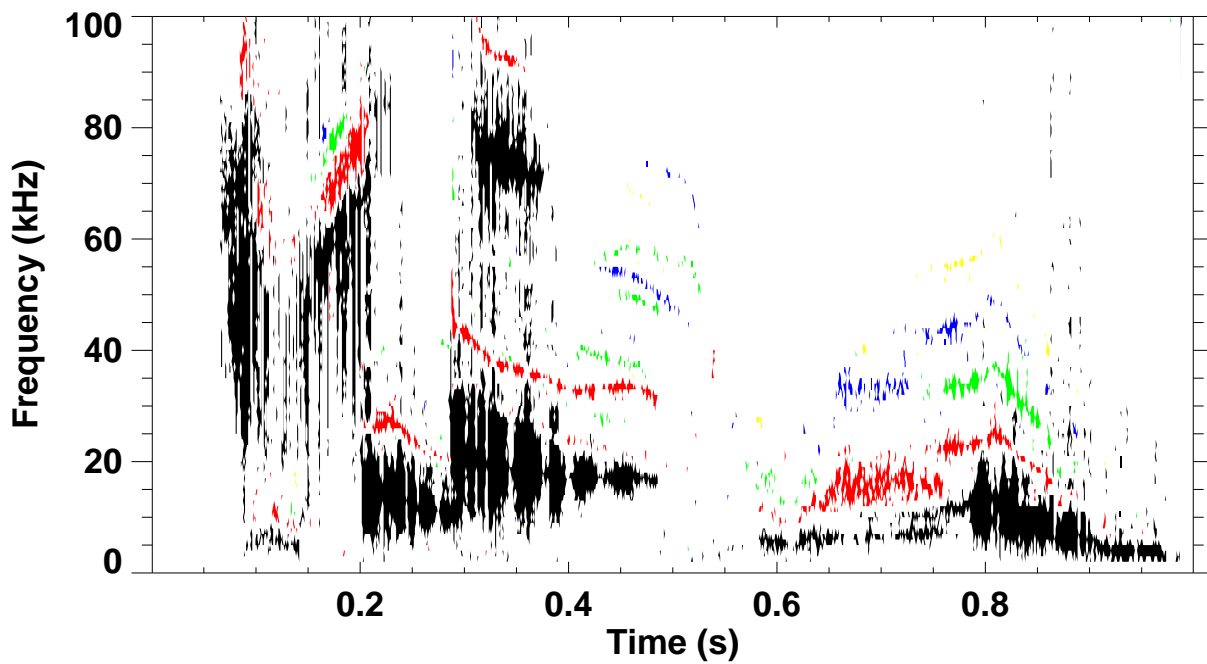
Shot 139612 \omega B(\omega) spectrum for toroidal mode number:
