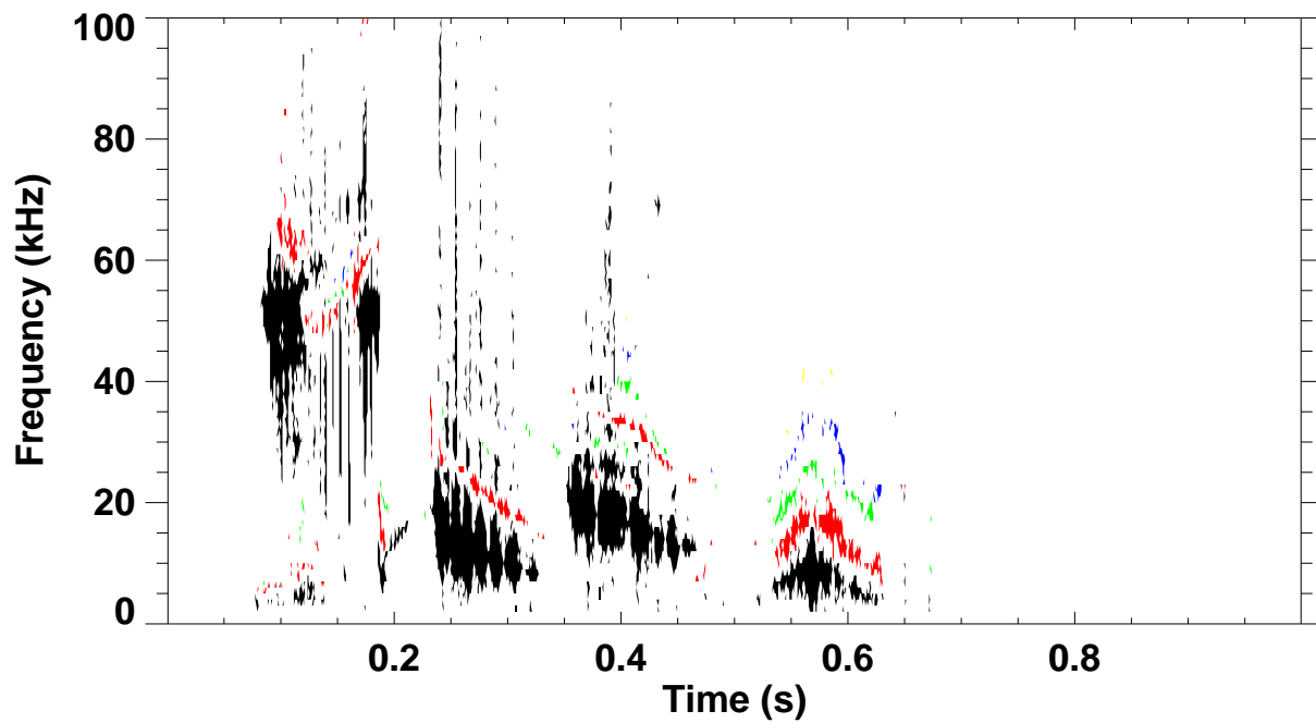
Shot 139995 \omega B(\omega) spectrum for toroidal mode number: 1 2 3 4 5
