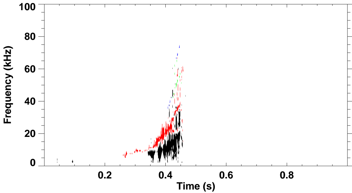
Shot 140184 \omega_B(\omega) spectrum for toroidal mode number: 1 2 3 4 5
