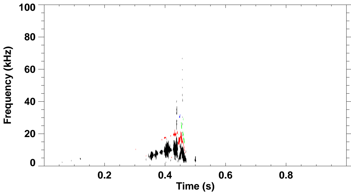
Shot 140189 \omega_B(\omega) spectrum for toroidal mode number: 1 2 3 4 5
