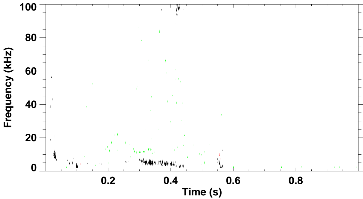
Shot 140230 \omega B(\omega) spectrum for toroidal mode number: 1 2 3 4 5
