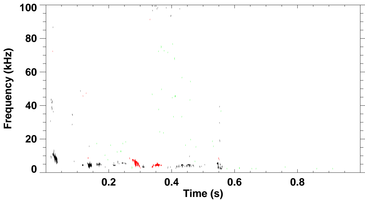
Shot 140241 \omega B(\omega) spectrum for toroidal mode number: 1 2 3 4 5
