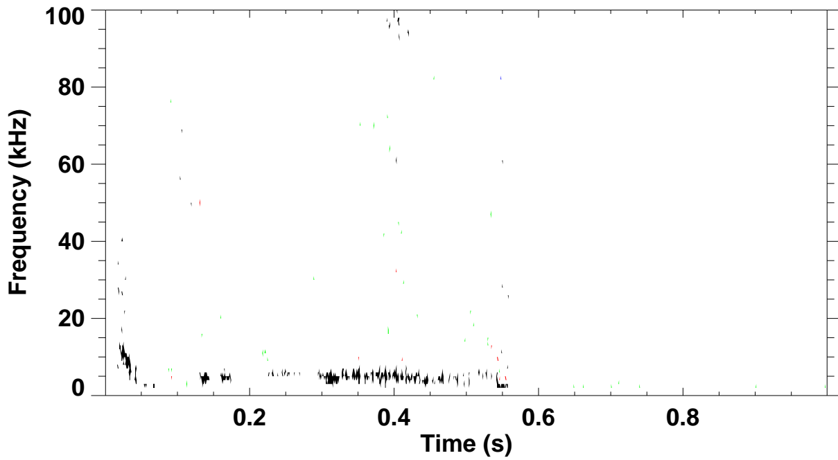
Shot 140247 \omega B(\omega) spectrum for toroidal mode number: 1 2 3 4 5
