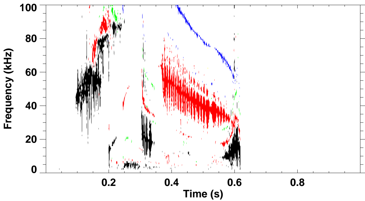
Shot 140273 \omega_B(\omega) spectrum for toroidal mode number: 1 2 3 4 5
