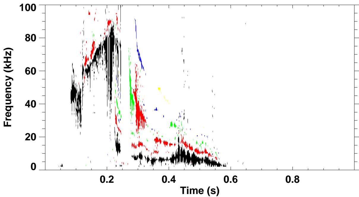
Shot 140278 \omega B(\omega) spectrum for toroidal mode number: 1 2 3 4 5
