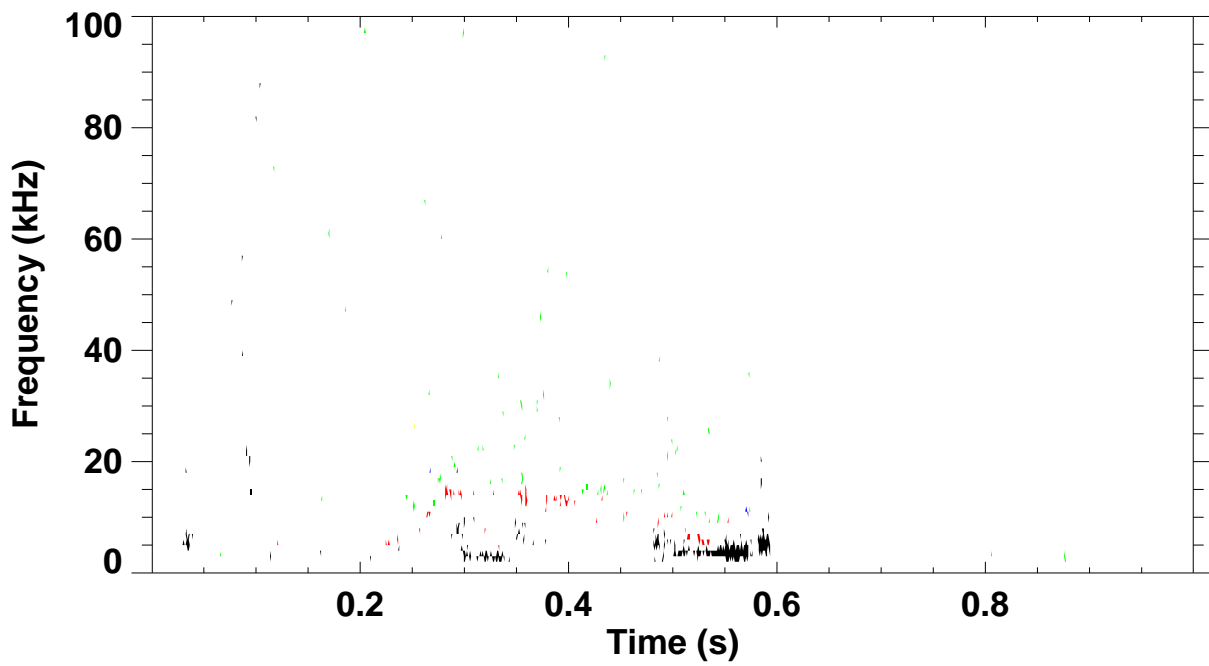
Shot 140296 \omega B(\omega) spectrum for toroidal mode number: 1 2 3 4 5
