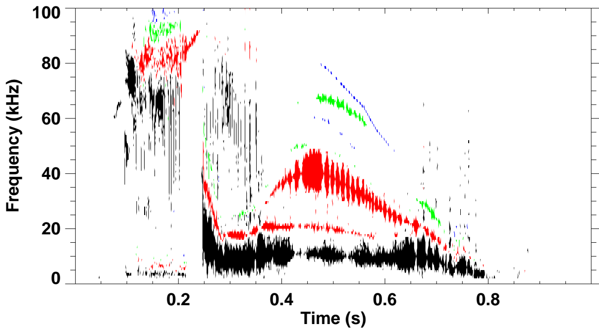
Shot 140612 \omega B(\omega) spectrum for toroidal mode number: 1 2 3 4 5
