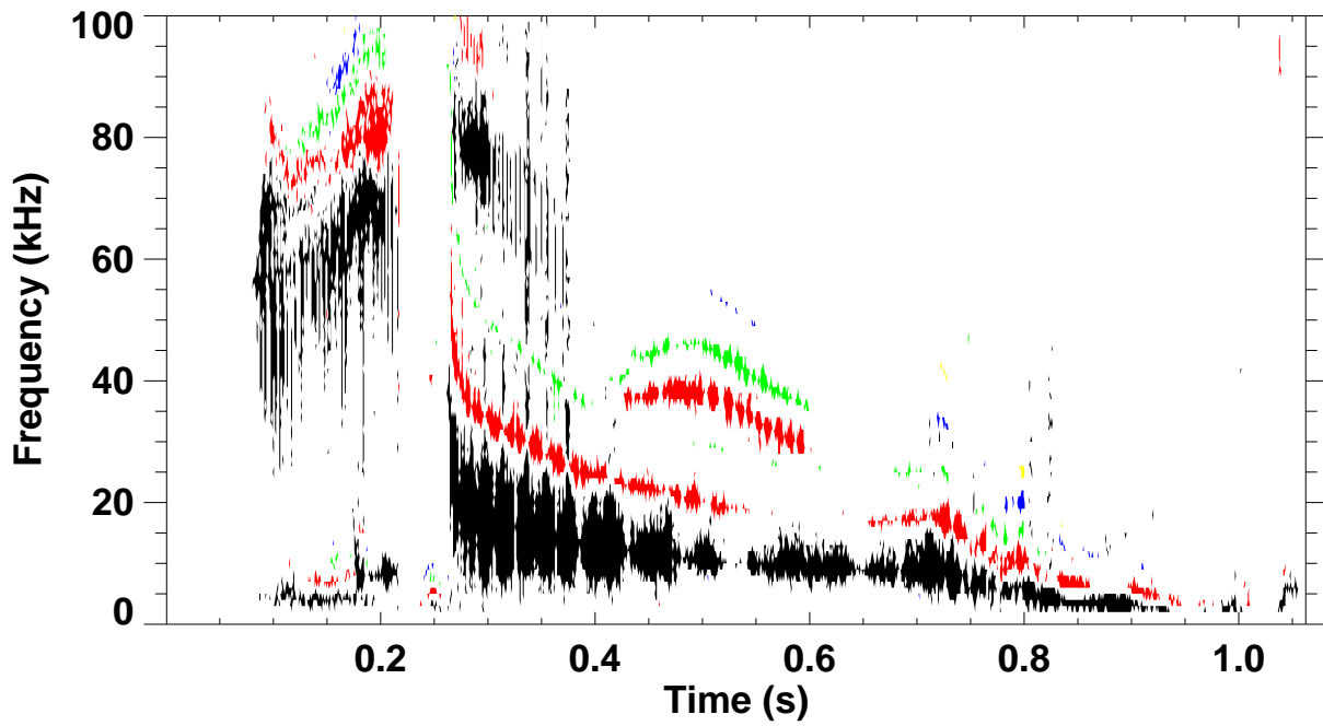
Shot 140617 \omega_B(\omega) spectrum for toroidal mode number: 1 2 3 4 5
