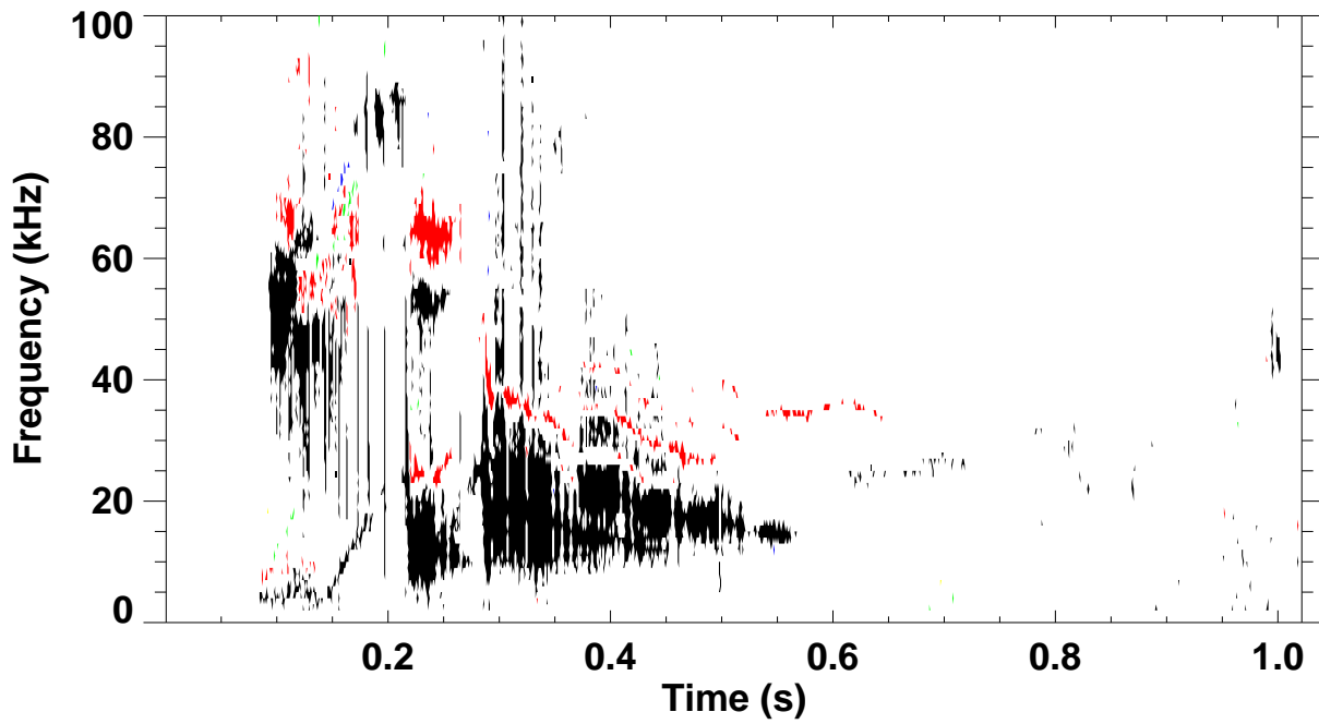
Shot 140711 \omega B(\omega) spectrum for toroidal mode number: 1 2 3 4 5
