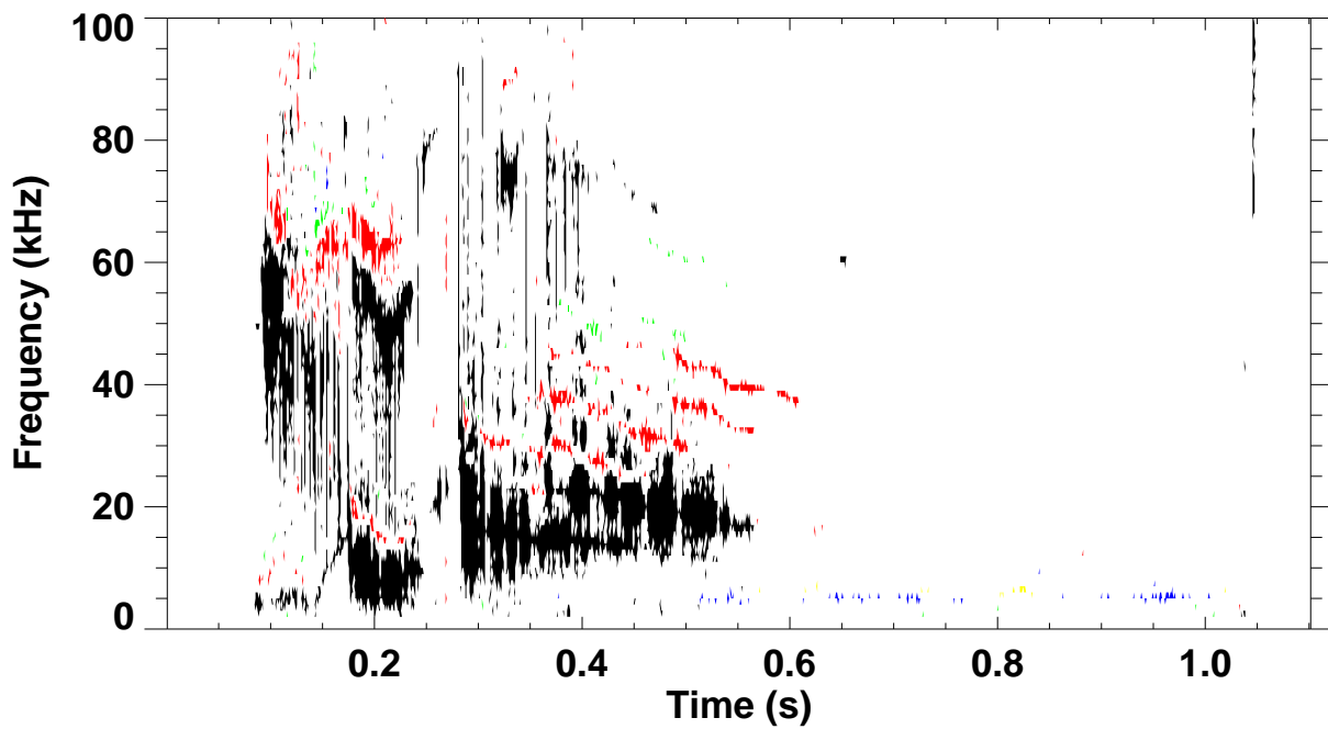
Shot 140738 \omega B(\omega) spectrum for toroidal mode number: 1 2 3 4 5
