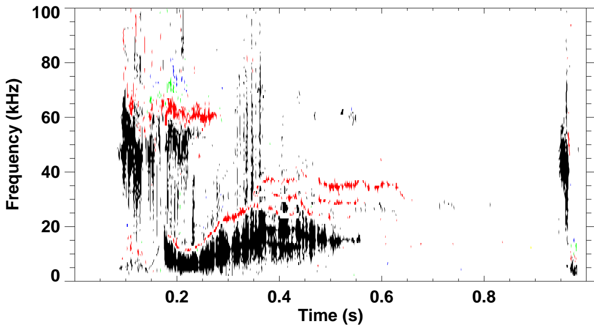
Shot 140741 \omega B(\omega) spectrum for toroidal mode number: 1 2 3 4 5
