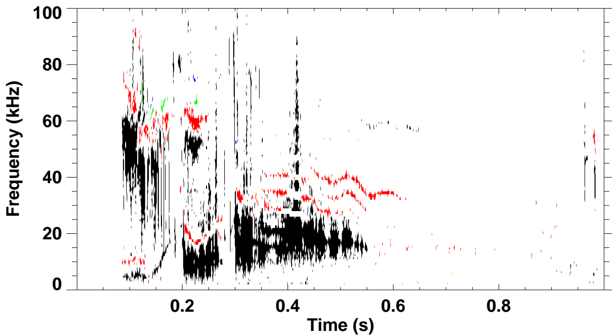
Shot 140749 \omega B(\omega) spectrum for toroidal mode number: 1 2 3 4 5
