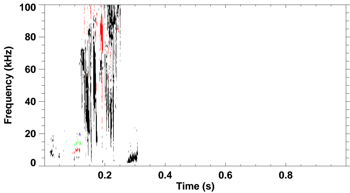
Shot 140872 \omega B(\omega) spectrum for toroidal mode number: 1 2 3 4 5
