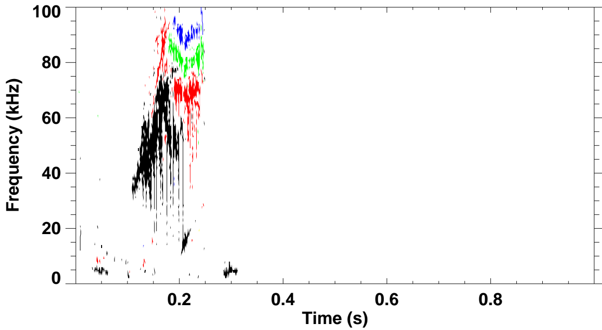
Shot 140937 \omega_B(\omega) spectrum for toroidal mode number: 1 2 3 4 5
