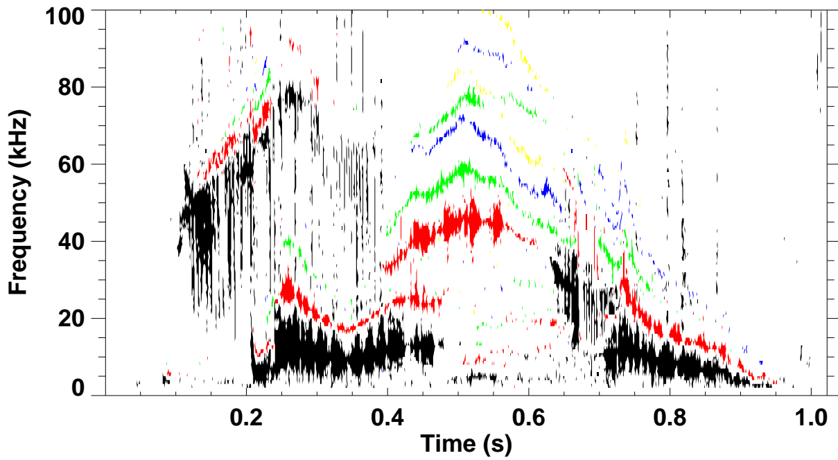
Shot 141268 \omega B(\omega) spectrum for toroidal mode number: 1 2 3 4 5
