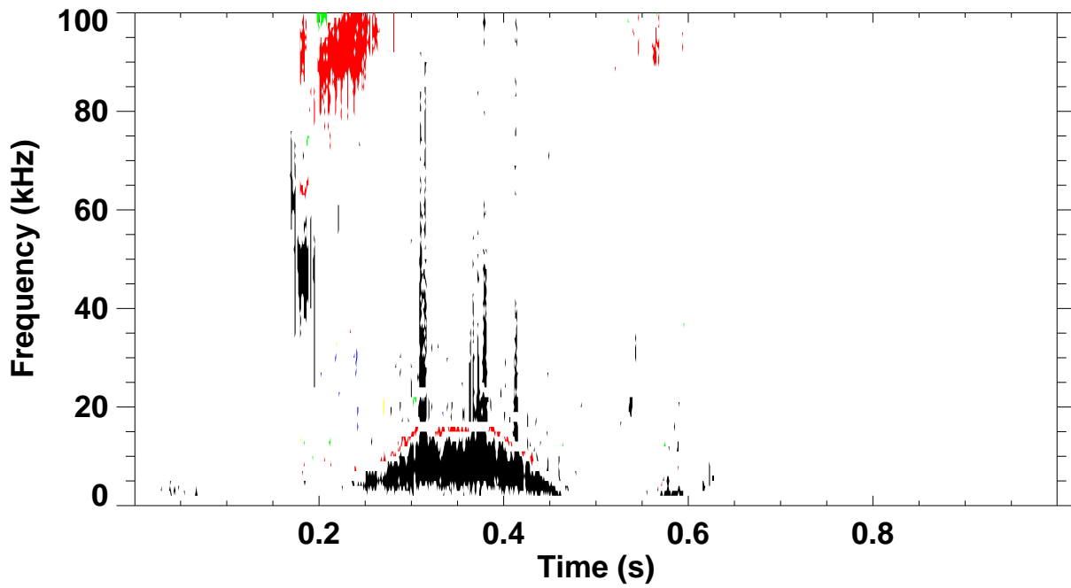
Shot 141291 \omega B(\omega) spectrum for toroidal mode number: 1 2 3 4 5
