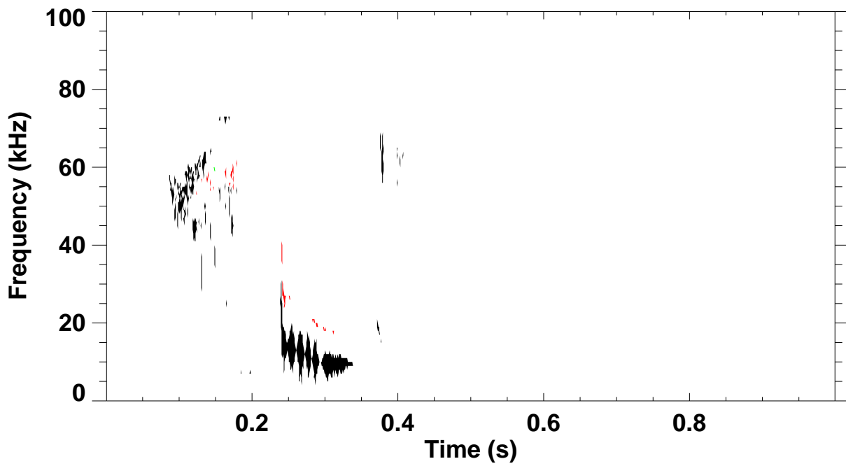
Shot 141561 \omega B(\omega) spectrum for toroidal mode number: 1 2 3 4 5
