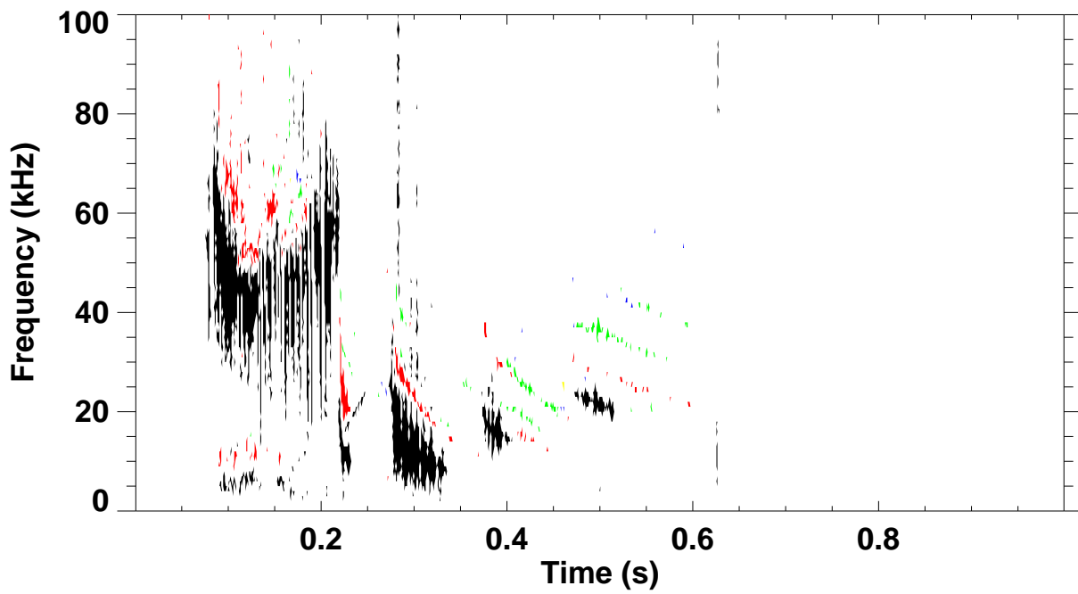
Shot 141581 \omega_B(\omega) spectrum for toroidal mode number: 1 2 3 4 5
