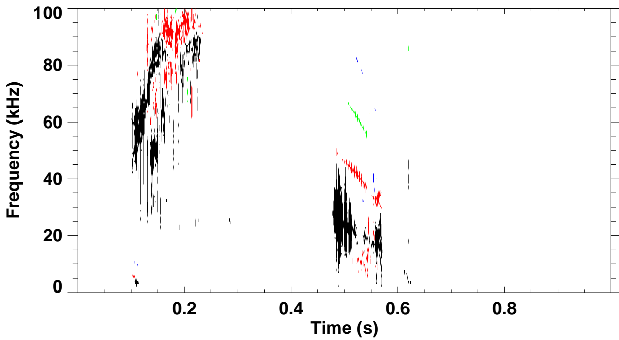
Shot 141720 \omega B(\omega) spectrum for toroidal mode number: 1 2 3 4 5
