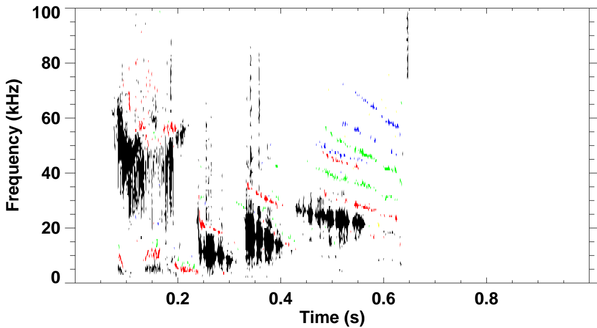
Shot 141760 \omega B(\omega) spectrum for toroidal mode number: 1 2 3 4 5
