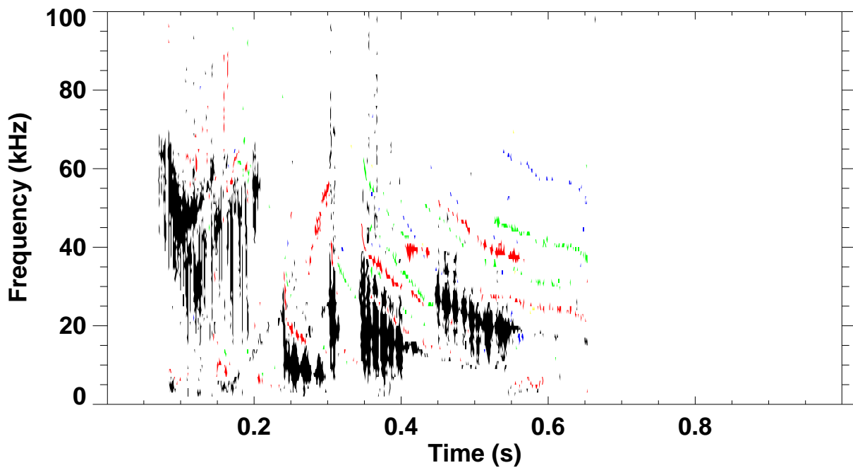
Shot 141766 \omega B(\omega) spectrum for toroidal mode number: 1 2 3 4 5
