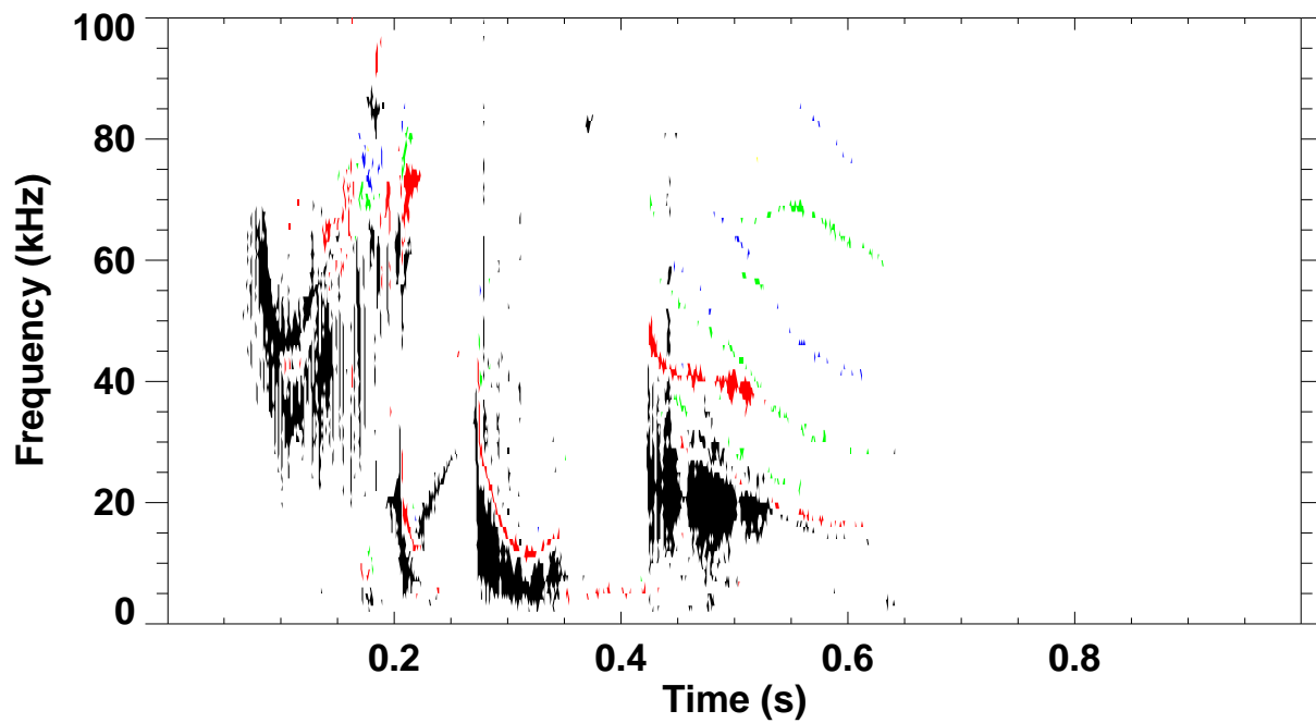
Shot 141775 \omega_B(\omega) spectrum for toroidal mode number: 1 2 3 4 5
