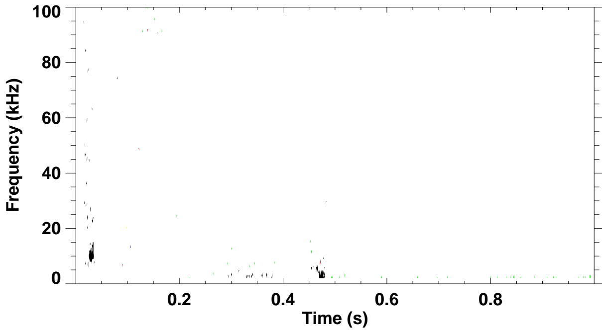
Shot 141798 \omega B(\omega) spectrum for toroidal mode number: 1 2 3 4 5
