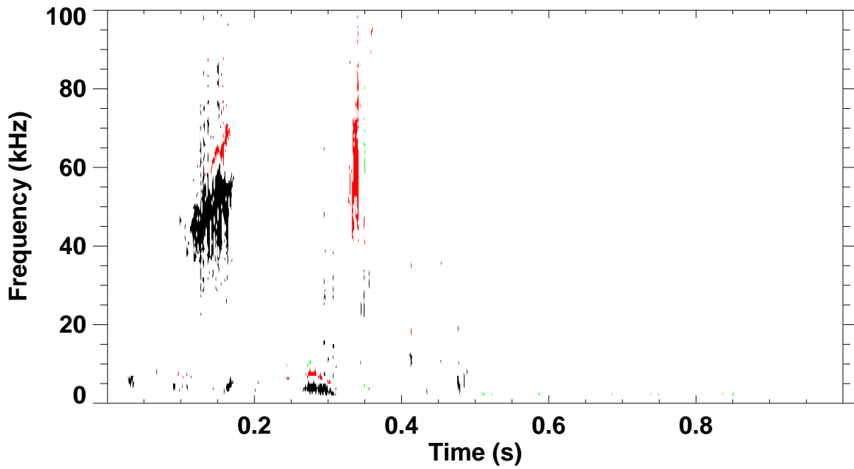
Shot 141918 \omega_B(\omega) spectrum for toroidal mode number: 1 2 3 4 5
