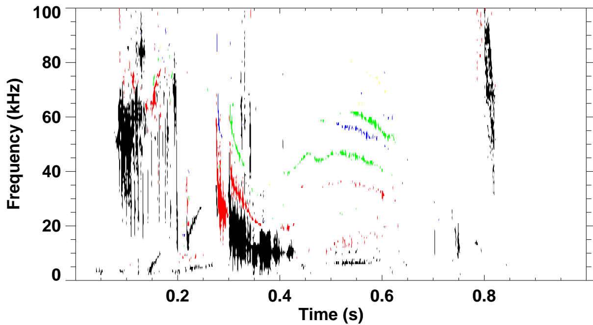
Shot 142012 \omega B(\omega) spectrum for toroidal mode number: 1 2 3 4 5
