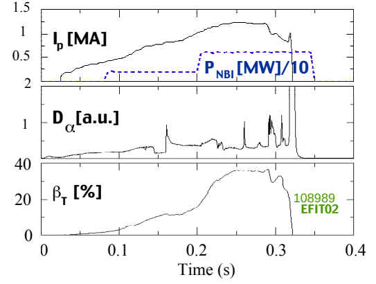
Figure 3. (a) Plasma current and NB power, (b). D_\alpha emission, and (c) \beta_T for a double-null plasma. The plasma had an applied toroidal field of 0.3 T, aspect ratio of 1.4, elongation of 2.0, triangularity of 0.8, internal inductance of 0.6, and a central q as determined from magnetics analysis of 1.4.
