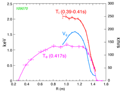
Figure 12. T_i , T_e , and toroidal rotation V_\phi in the long pulse H mode discharge described in Figure 4.
