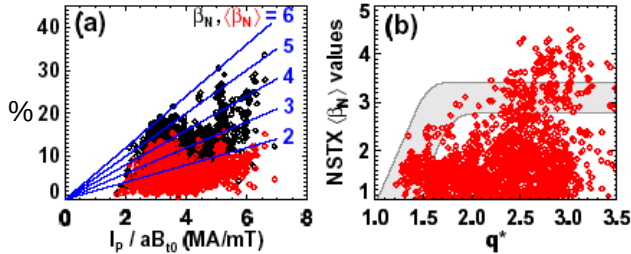
Figure 8. (a) \beta_T (black) and \langle\beta\rangle (red) at maximum stored energy for NBI-heated plasmas plotted versus normalized current. Constant \beta_N lines are shown (b) \langle\beta_N\rangle versus q^* for the discharges from (a). From Ref. 25.
