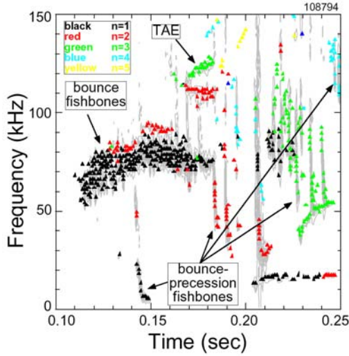
Figure 9. A sampling of the energetic particle modes often observed an NSTX neutral-beam-heated discharge.
