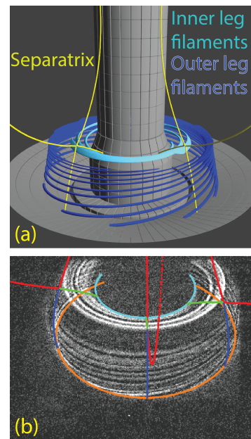
Figure 7: (a) Rendering of the NSTX-U divertor with flux tubes corresponding divertor-localized fluctuations; (b) Divertor image in C III emission ( 9 \mu\text{s} exposure) after high pass filtering. Separatrix (red), inner (green) and outer (blue) divertor legs, inner (cyan) and outer (orange) strike points are overlaid.
