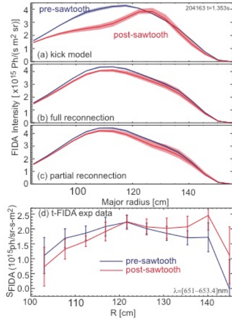
Fig. 5 Comparison of t-FIDA spatial profiles calculated by FIDASim using the plasma profiles and fast ion distribution from (a) the kick model, (b) the Kadomstev full reconnection model, (c) the Porcelli partial reconnection model. The measured t-FIDA profiles are shown in (d).
