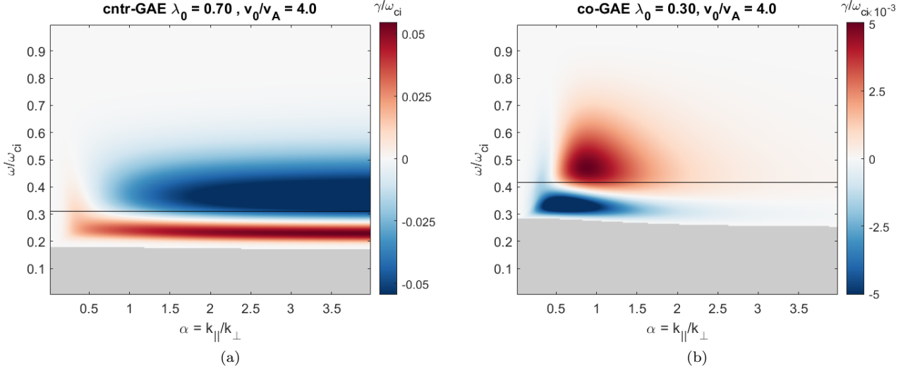
FIG. 4. Numerically calculated fast ion drive/damping for GAEs as a function of \bar{\omega} = \omega/\omega_{ci} and \alpha = |k_{\parallel}/k_{\perp}| , when driven by a beam distribution with (a) \lambda_0 = 0.7 for cntr-GAEs and (b) \lambda_0 = 0.3 for co-GAEs. Also, v_0/v_A = 4.0 , \Delta\lambda = 0.3 , and assuming \langle \bar{\omega}_{ci} \rangle \approx 0.9 . Red corresponds to net fast ion drive, blue to damping, and gray to regions excluded by the resonance condition. Black line is the marginal frequency for fast ion drive predicted by the approximate analytic conditions in Eq. 40 and Eq. 41.
