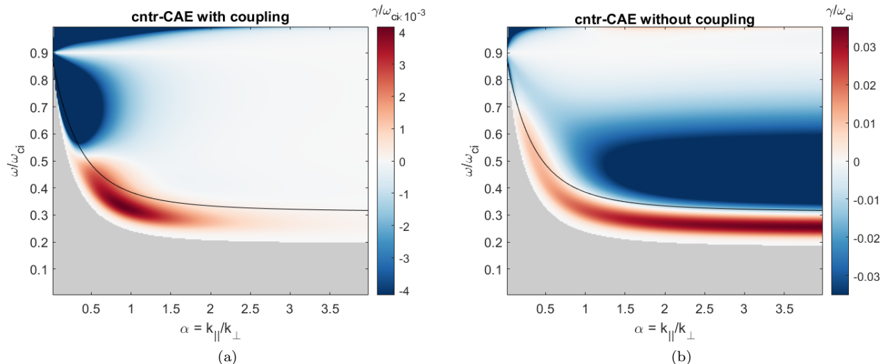
FIG. 5. Numerically calculated fast ion drive/damping for cntr-CAEs as a function of \bar{\omega} = \omega/\omega_{ci} and \alpha = |k_{\parallel}/k_{\perp}| when coupling to the shear branch is (a) included and (b) neglected. In both calculations, the modes are driven by a beam distribution with \lambda_0 = 0.7 , v_0/v_A = 4.0 , \Delta\lambda = 0.3 , and assuming \langle \bar{\omega}_{ci} \rangle \approx 0.9 . Red corresponds to net fast ion drive, blue to damping, and gray to regions excluded by the resonance condition. Black line is the marginal frequency for fast ion drive predicted by the approximate analytic condition in Eq. 42.
