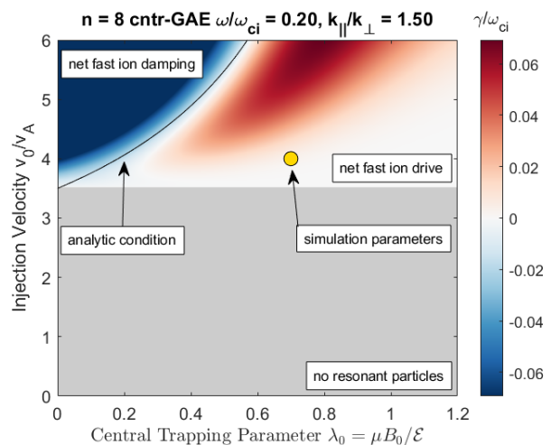
FIG. 2. Numerical integration of full growth rate expression Eq. 21 as a function of fast ion distribution parameters v_0/v_A and \lambda_0 with \Delta x = 0.30 for a ctr-GAE with properties inferred from HYM simulations: \omega/\omega_{ci} = 0.20 and |k_{\parallel}/k_{\perp}| = 1.50 , implying \zeta = 0.47 . Red indicates net fast ion drive, blue indicates net fast ion damping, and gray indicates beam parameters with insufficient energy to satisfy the resonance condition. Black curve shows approximate stability condition derived in Eq. 30.
