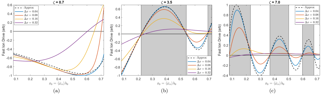
FIG. 1. Comparison of numerically integrated growth rate to narrow beam approximation for ctr-GAE with \eta = 0.2 as a function of the central trapping parameter of the beam distribution. Black dashed line shows the analytic approximation made in Eq. 26 for \Delta x = 0.04 and (a) \zeta = 0.7 , (b) \zeta = 3.5 , and (c) \zeta = 7.0 . Colored curves show numerical integration of Eq. 24 for different values of \Delta x : blue \Delta x = 0.04 , orange \Delta x = 0.08 , gold \Delta x = 0.16 , and purple \Delta x = 0.32 . Shaded regions correspond to regions of drive according to the narrow beam approximation.
