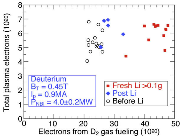
Fig. 3. A database of total plasma electrons versus total electrons of the injected deuterium gas fuel showing Li edge conditions require large fueling increases to maintain density and constant discharge conditions.
