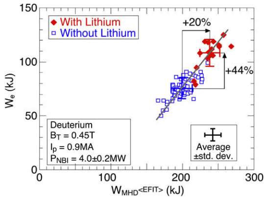
Fig. 4. A database of electron stored energy ( W_e ) versus total stored energy ( W_{\text{MHD}} ) for deuterium reference plasmas immediately following Li deposition, and for deuterium reference plasmas prior to Li deposition showing stored energy increases after Li deposition mostly through increase in electron stored energy. The EFIT equilibrium analysis is constrained by external magnetics, electron profile shape, and diamagnetic flux.
