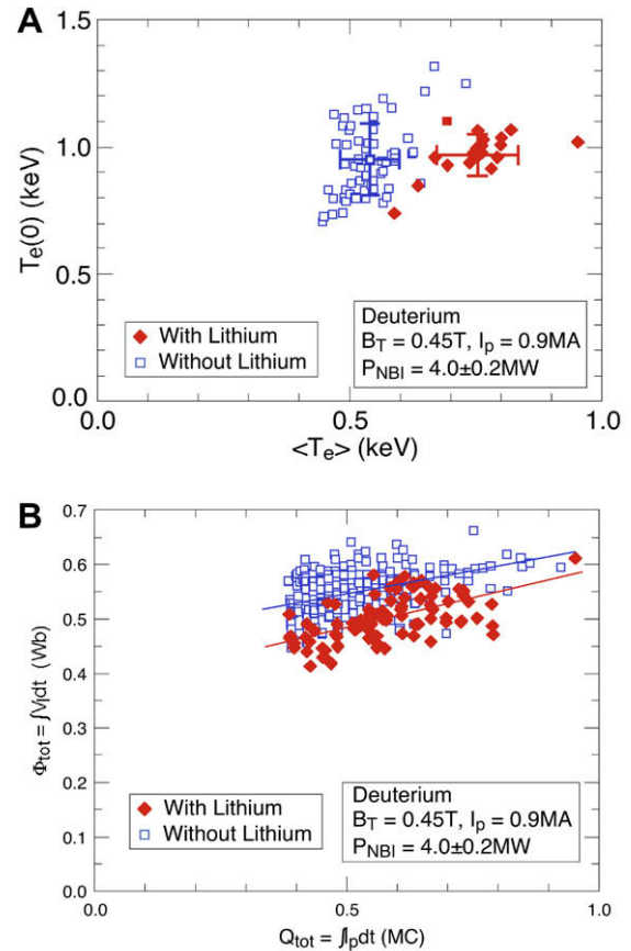
Fig. 5. (A) A database of central electron temperature ( T_e(0) ) versus average electron temperature ( \langle T_e \rangle ) at the time of peak ( T_e ), with and without Li edge conditions, and (B), shows for the same discharges at the time of peak ( T_e ), the integrated loop voltage (Wb) versus the integrated toroidal current (MC). In (B) the solid lines are a guide to the eye.
