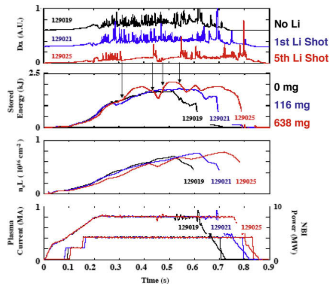
Fig. 6. Comparison for pre-Li and post-Li reference shots showing Li edge conditions mitigate ELMs, increase stored energy, and lengthen pulse.
