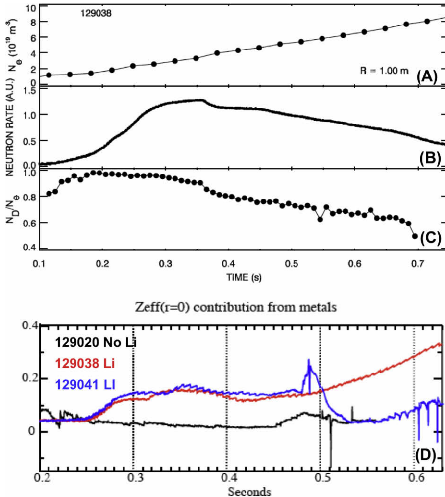
Fig. 8. (A) central density, (B) neutron rate, and (C) ratio of core deuterium density ( N_D ) to central electron density, and (D) Z-effective show that during Li edge conditions, as core deuterium-to-central density ratio decreases and neutron rate decreases.
