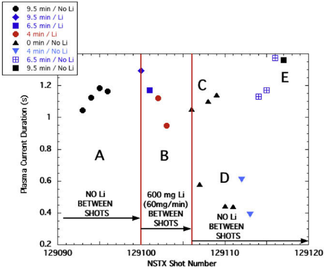
Fig. 7. Shown are the effects on H-mode pulse length of varying amounts of applied HeGDC duration and Li deposition. (A) Reference shots were taken following 9.5 min of HeGDC and no Li between shots. (B) The HeGDC shortened from 9.5 to 4 min followed by 10 min Li deposition. (C) No HeGDC and no Li deposition were performed between discharges. Initially there was no change at (C) no change, but by (D) conditions degrade. Reapplication of HeGDC (E) restored and exceeded initial conditions (A).
