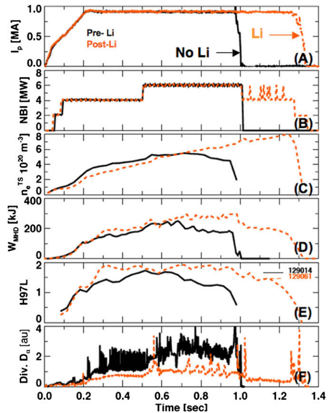
Fig. 2. Comparison for pre-Li and post-Li reference shots with constant NBI, constant external gas, and operating parameters showing how Li edge conditions reduce ELMs (F), and increase confinement (E), stored energy (D), and pulse length (A).
