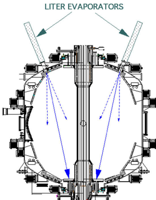
Fig. 1. Schematic diagram of the poloidal cross section of NSTX, the locations of the two LITHium EvaporatoRs (LITERs) at toroidal angles 165° and 315°, and the LITER central-axis aimed at the lower divertor, and dashed lines indicating the gaussian half-angles at 1/e intensity of the measured evaporated Li angular distributions.
