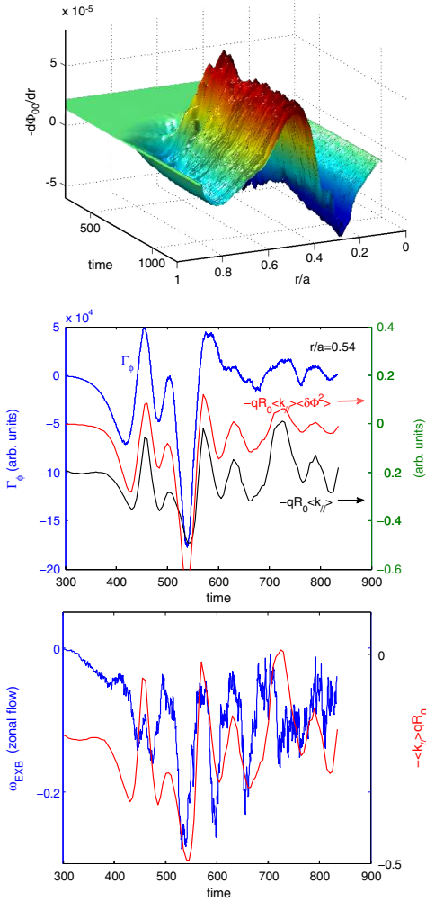
FIG. 3 (color online). Spatiotemporal evolution of zonal flow (top), time history of \Gamma_\phi , -\langle k_{\parallel} \rangle and -\langle k_{\parallel} \rangle \langle \delta\Phi^2 \rangle (middle) and zonal flow \omega_{EXB} and -\langle k_{\parallel} \rangle (bottom), showing residual stress generation due to zonal flow shear.
