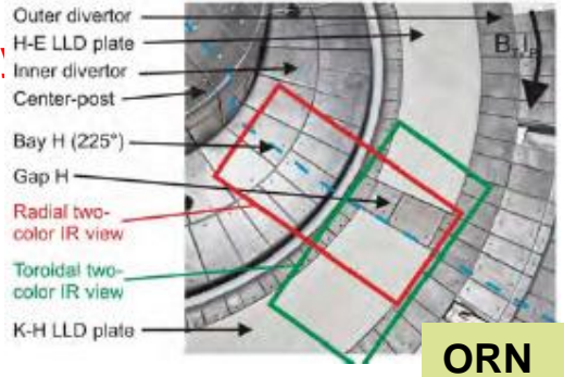
Dual-band fast IR Camera
