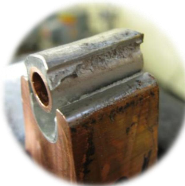
Solder paste injection over cooling tube
