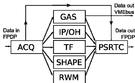
Figure 4 Real-time information flow chart for the NSTX control system
