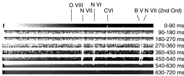
FIG. 1. Sequence of 1340 \times 10 pixel spectral images obtained with XEUS for NSTX shot 123 629. The locations of the dominant K -shell lines of boron, carbon, nitrogen, and oxygen are marked.
