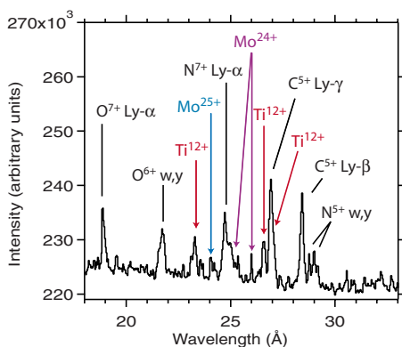
FIG. 4. (Color online) Spectral emission recorded with XEUS during shot 123 721. Lines not normally seen in the spectrum are tentatively ascribed to the 1s^2 2s^2 2p^3 3s \rightarrow 1s^2 2s^2 2p^6 and 1s^2 2s^2 2p^5 3d \rightarrow 1s^2 2s^2 2p^6 transitions in neonlike Ti XIII and to 4d \rightarrow 3p transitions in argonlike and chlorinelike Mo XXV and Mo XXVI.
