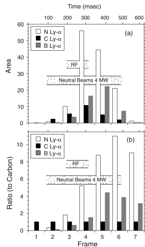
FIG. 3. Time-dependent emission of the Lyman- \alpha lines of B v, C vi, and N vii during NSTX shot 123 629: (a) absolute intensities and (b) intensities relative to the C vi emission.
