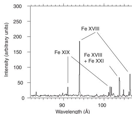
FIG. 5. Spectral emission recorded with XEUS during shot 120 220. Lines are identified to originate from iron ions and are labeled by the emitting ion.
