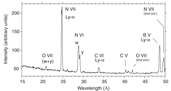
FIG. 2. K -shell emission features observed with XEUS in frame 7 during NSTX shot 123 629. Lines are labeled by the emitting ion. \text{Ly-}\alpha denotes the 2p \rightarrow 1s transition in hydrogenlike ions; w and y denote the 1s2p^3P_1 \rightarrow 1s^2^1S_1 resonance and the 1s2p^3P_1 \rightarrow 1s^2^1S_1 intercombination transition, respectively.
