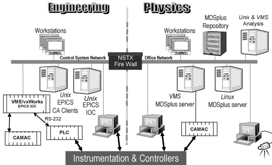
Fig. 1. The NSTX Data Acquisition and Control System.
