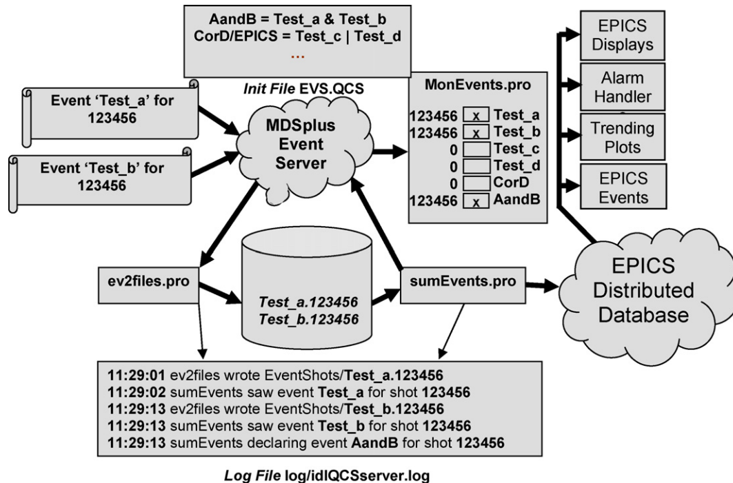
Fig. 2. The Event Summation System for MDSplus.
