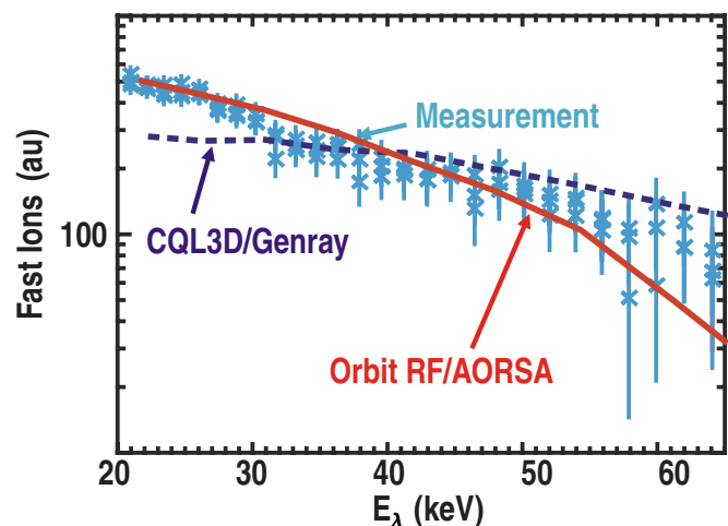
FIG. 12. (Color online) Fast-ion spectra from FIDA (signal \times with error bar), CQL3D/GENRAY (dashed line) and ORBIT-RF/AORSA (solid line) for NSTX 128739 high harmonic ICRF heating discharge. Here, E_\lambda is the component of fast-ion velocity along vertical collection lens.
