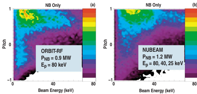
FIG. 6. (Color online) Contour plots of fast beam-ion distributions computed from (a) ORBIT-RF and (b) NUBEAM for DIII-D 122993 before ICRF heating turns on.
