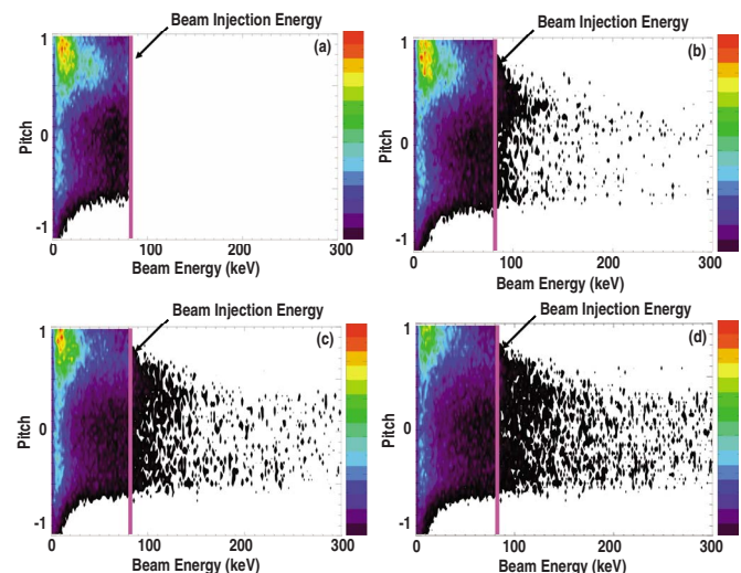
FIG. 9. (Color online) Contour plots of fast-ion distribution computed from ORBIT-RF coupled with AORSA (a) before ICRF wave turns on, (b) at 20 ms after ICRF turns on, (c) at 70 ms after ICRF turns on, and (d) at 160 ms after ICRF turns on, for DIII-D 122993, indicating that beam tails are being created above the beam injection energy 80 keV during ICRF heating.
