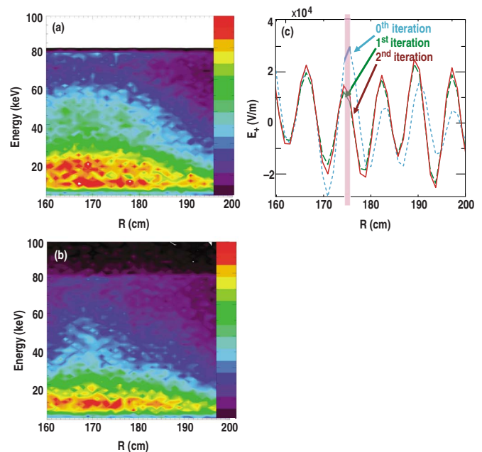
FIG. 8. (Color online) Contour plots of fast beam-ion distribution computed from ORBIT-RF (a) before ICRF wave turns on, (b) after ICRF wave turns on, and (c) E_+ component of ICRF wave electric field computed from AORSA at zeroth iteration (dot), first iteration (dash), and second iteration (solid), for DIII-D 122993 heating parameters.
