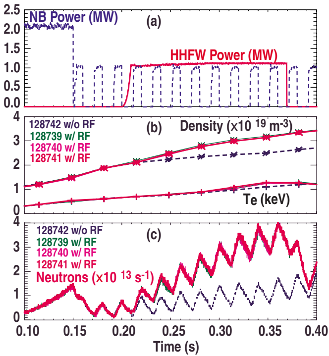
FIG. 3. (Color online) Time traces of experimental data from NSTX ICRF heating discharges (128739–128741) and no ICRF discharge (128742) for eighth harmonic central damping of 30 MHz ICRF wave on injected beam ions (a) beam injection power (dash) and ICRF wave power (solid), (b) central electron density (ICRF shots for solid with symbol ★, no ICRF shot for dash with symbol +) and central electron temperature (ICRF shots for solid with symbol +, no ICRF shot for dash with symbol +), and (c) measured neutron rates from three identical ICRF shots (solid) and one no ICRF shot (dash).
