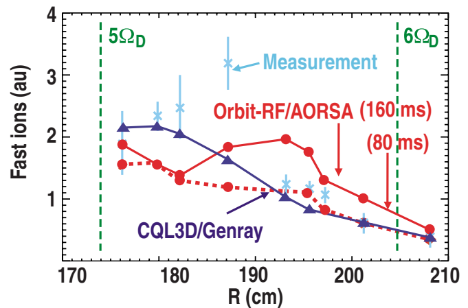
FIG. 11. (Color online) Fast-ion spatial profiles from FIDA (signal \times with error bar), CQL3D/GENRAY (solid with \blacktriangle ), ORBIT-RF/AORSA (dashed line with \bullet for 80 ms simulation and solid line with \bullet for 160 ms simulation) for DIII-D 5 th harmonic ICRF heating discharge 122793. Here, vertical dotted lines are fifth and sixth harmonic resonance layers of injected deuterium beam ions.
