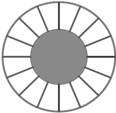
Fig. 1. Horizontal cross-section view of the center portion of the all-metal center stack. The central region is ferritic material, surrounded by copper wedges, which are in turn separated by resistive inserts.
