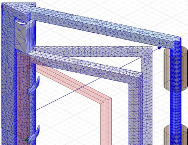
Fig. 3. Close up view of the sector model showing the discretization of the material.
