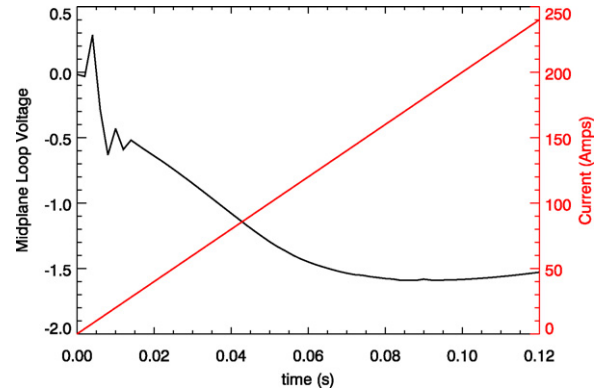
Fig. 4. Time history of the applied current waveform in the external coils (in red). Resultant voltage waveform on the device midplane. The loop voltage reaches 1.5 V, which should be enough to achieve plasma breakdown and ramp up (in black). (For interpretation of the references to color in this figure legend, the reader is referred to the web version of the article.)
