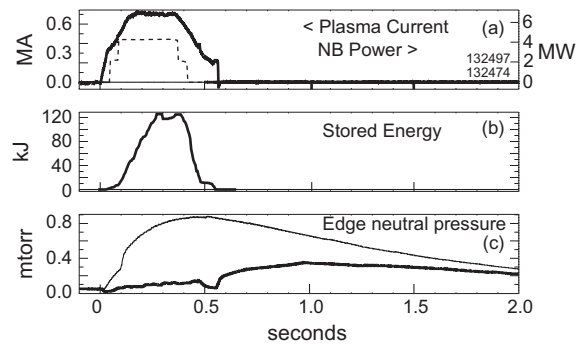
Fig. 2. (a) Plasma current, (b) stored energy and (c) in-vessel pressure for gas-only ‘shot’ (thin line), and NB heated discharge (thick line) before lithium conditioning. The gas fueling was programmed to be the same in both cases. The NB power is shown dashed.
