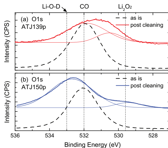
Fig. 5. XPS O1s spectra from two graphite samples showing 533.0 eV peak associated with retention of D in lithiated graphite matrix. PMI probe sample ATJ 150p (lower pane (b)) has about 10 more times lithium deposition than sample ATJ 139p (upper pane (a)). The thin lines represent multiple peaks that compose the primary peak. The dashed lines are the spectra before Ar cleaning.
