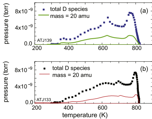
Fig. 6. Thermal desorption spectra (TDS) of ATJ graphite samples exposed via the PMI probe to 6 NB heated NSTX discharges with-, (a), and without-, (b), lithium exposure. The mass = 20 peak is plotted separately and corresponds to emission of D_2O .
