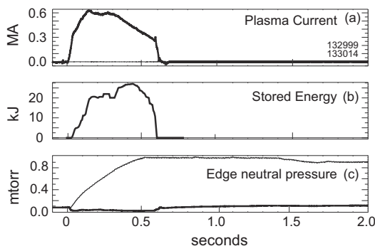
Fig. 1. (a) Plasma current, (b) stored energy and (c) in-vessel pressure for gas-only ‘shot’ (thin line), and ohmic discharge (thick line) with lithium conditioning.
