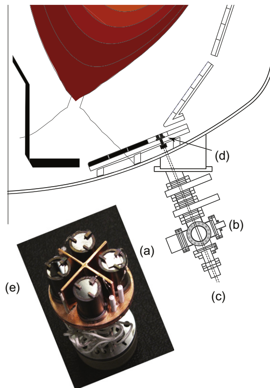
Fig. 4. Probe configuration on the lower NSTX vessel with magnetic flux lines for a low triangularity plasma. The chamber has been rotated 90^\circ to show: (a) port for residual gas analyzer or sample insertion, (b) pumping port, (c) probe drive and (d) probe head. An image of the probe head with four samples is shown in insert (e).
