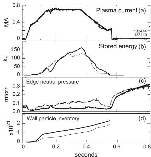
Fig. 3. (a) Plasma current, (b) stored energy, (c) in-vessel pressure and (d) wall inventory calculated by dynamic particle balance model for pre-Li (thin line), and with-Li (thick line) NB heated discharges.
