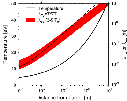
Fig. 1. Plot showing temperature and the temperature-gradient scale-length as a function of distance from the PFC surface for a conduction limited SOL profile. The target plasma is 4 eV at 4e20 \text{ m}^{-3} which yields \approx 4 \text{ MW/m}^2 at 5^\circ angle of incidence, similar to divertor plasmas measured in this study. The red band indicates the electron–electron mean-free-path for electrons with mean energy of 3–5 T_e . (For interpretation of the references to color in this figure legend, the reader is referred to the web version of this article.)
