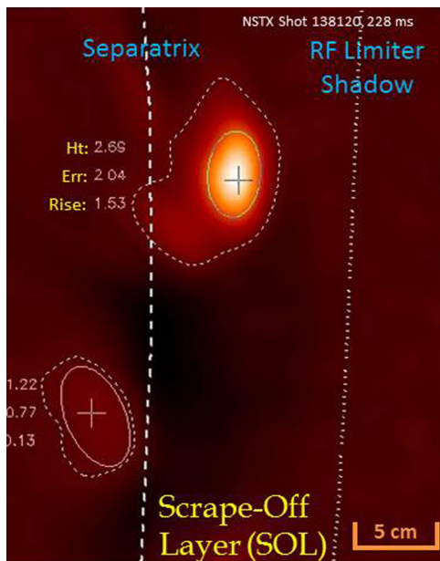
Fig. 2. An example of a analyzed blobs from a false-color image from the GPI camera. The separatrix position, taken from EFIT equilibrium reconstructions, is shown by a dashed line and the limiter shadow is shown by a dotted line. The solid ellipses indicate a fit to a contour line midway between the base and top of the blob region.
