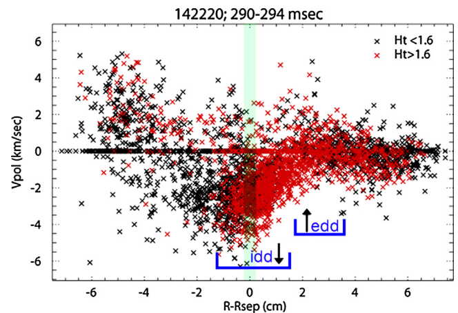
Fig. 4. Poloidal velocity vs. distance from the separatrix plotted for all blobs detected over 4 ms for NSTX shot 142,220. Larger than average blobs are in red, smaller ones in black. Blue lines indicate the ion drift direction (idd) and electron drift direction (edd) to show how the shear reverses from the -1 \text{ cm} to 2 \text{ cm} region and between 2 \text{ cm} and 4 \text{ cm} . Note that there are many more large blobs outside the separatrix. The green area indicates the separatrix region.
