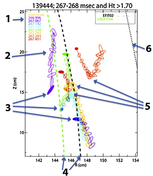
Fig. 3. Output from BlobTrails.html showing blob history for 1 ms on NSTX shot 139,444. Indicated are (1) the starting times of the blobs tracked, (2) the tilt and elongation from fitting an ellipse (relative size can be shown, but is not in this example), (3) the starting location of blob trails are indicated by a filled ellipses, (4) the location of the separatrix predicted by LRdfit (green online), and EFIT (black), (5) sheared flow indicated by changes in direction, and (6) the location of the limiter shadow. “Ht > 1.70” means that only blobs with a normalized intensity 70% higher than the average are shown.
